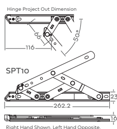
SPT10 Right Hand Shown, Left Hand Opposite.
