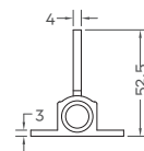
Top Profile
