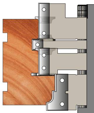
TRITUS FRAME TOOLING BLOCK EXAMPLE
