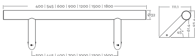
Side Profile
