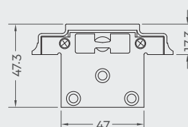
Front Profile
