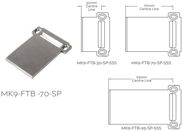
MK9-FTB Adjustable Striker Plate
