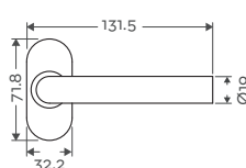
Front Profile
