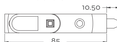
Front Profile
