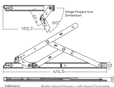
SPSH16 Right Hand Shown, Left Hand Opposite.
