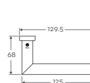
Top Profile
