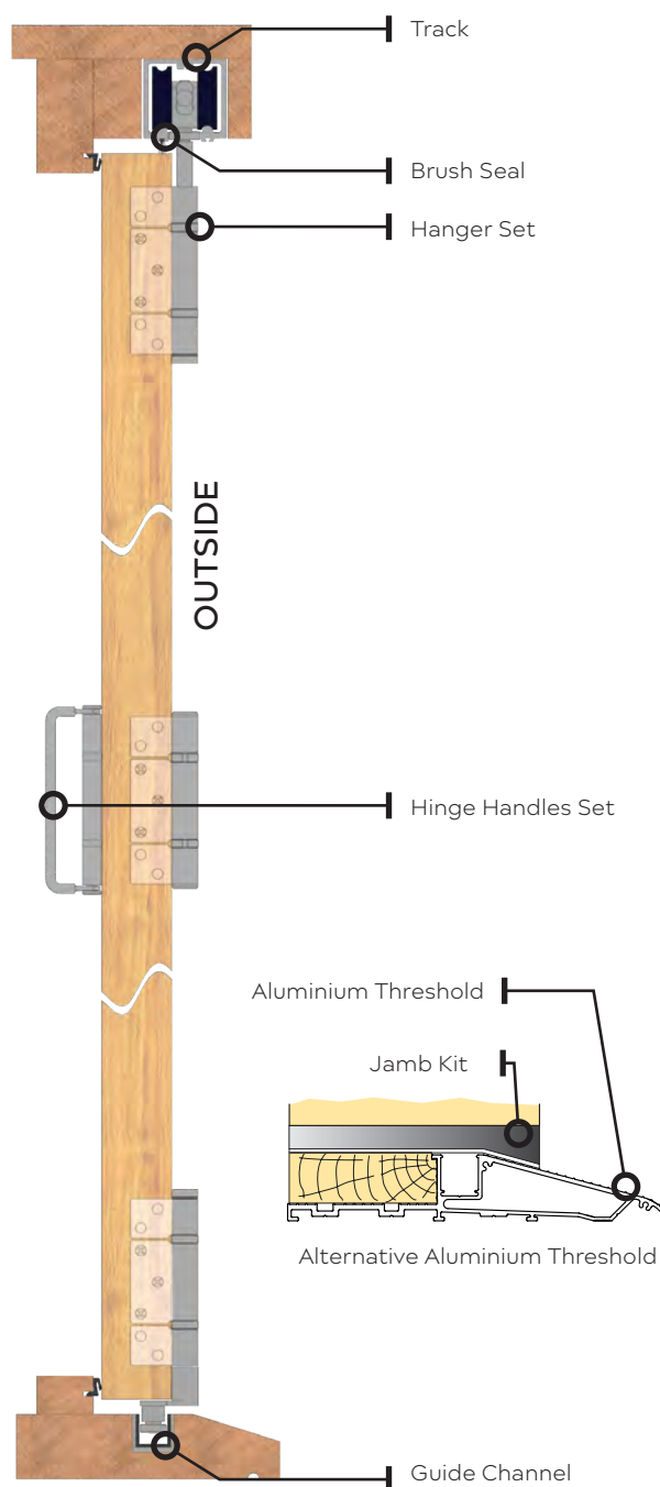
Securefold Pro Side Section
