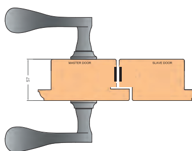
SINGLE HANDLE (SOLO)
