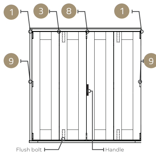
TYPICAL OUTSIDE ELEVATION
