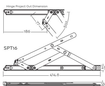
SPT16 Right Hand Shown, Left Hand Opposite.
