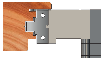
Multipoint Lock Groove
