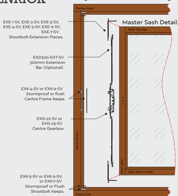
Single Casement Window Configuration.
