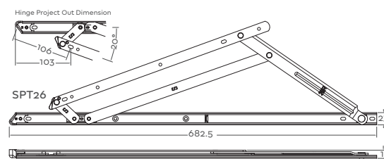
SPT26 Right Hand Shown, Left Hand Opposite.
