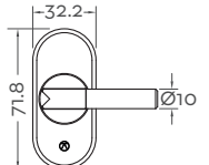
Front Profile
