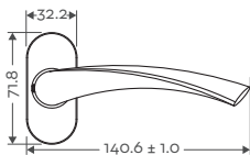
Front Profile
