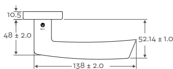
Top Profile
