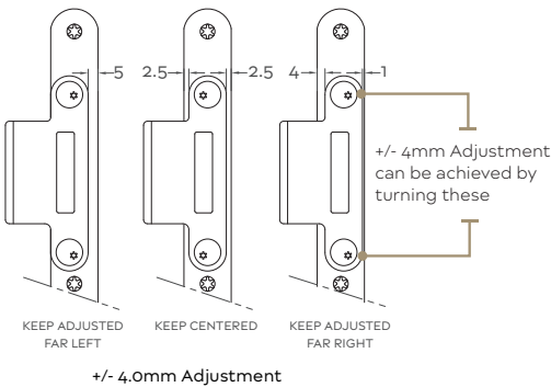
MK9 ADJUSTMENT POINTS
