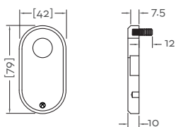
External Security Escutcheon (used in SE40A & SE40B)
