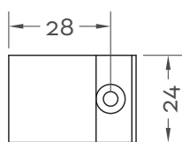
Top Profile
