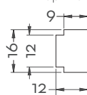
Top Profile
