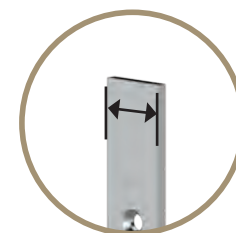
Square End ML4120S - 20mm Faceplate ML4126S - 16mm Faceplate
