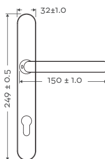
Front Profile
