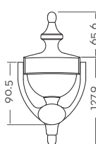
Front Profile
