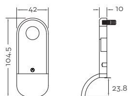
Internal Escutcheon (used in SE40B & SE40C)
