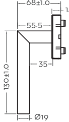
Side Profile
