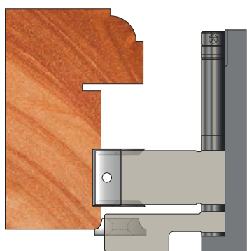
One-Piece Keep
