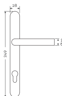
Front Profile
