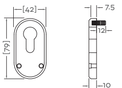
External Security Cylinder Pull (used in SE40C & SE40D)
