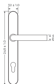
Front Profile
