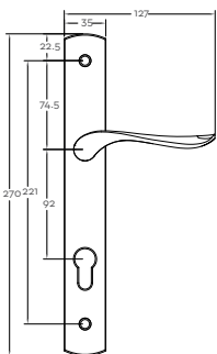
Front Profile
