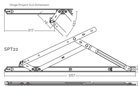
SPT22 Right Hand Shown, Left Hand Opposite.
