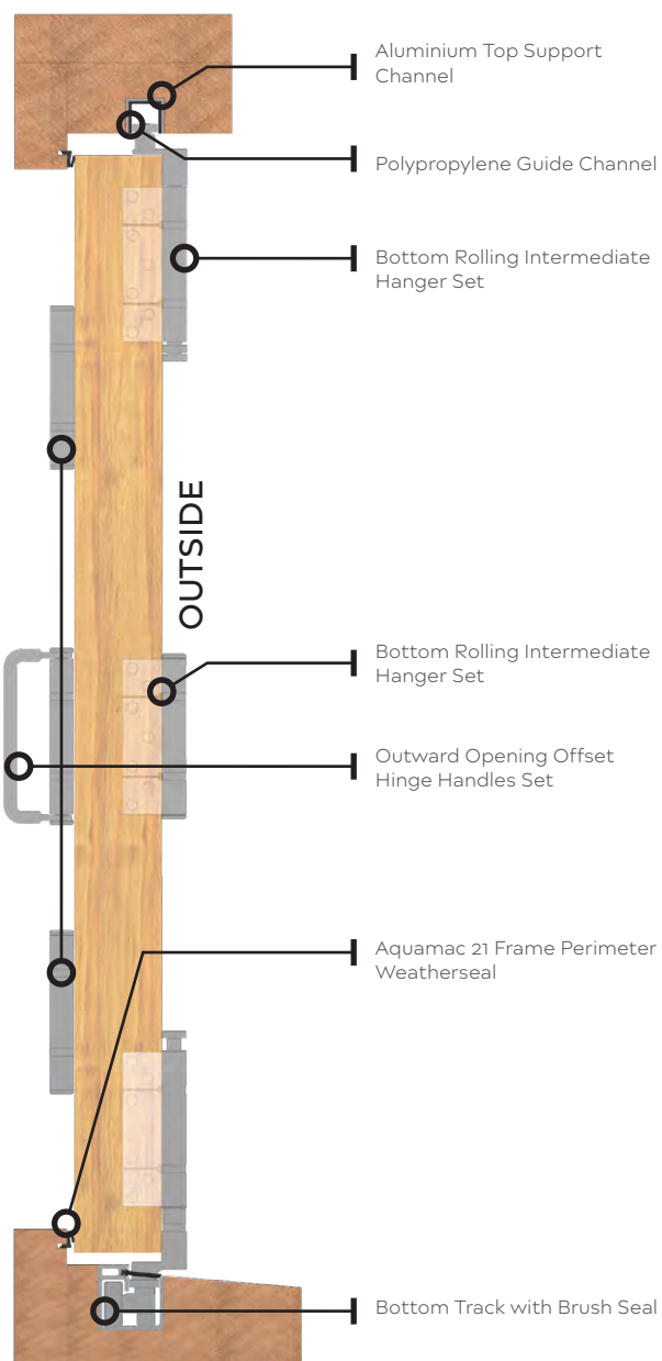
SECUREFOLD Side Section
