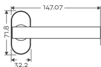
Front Profile
