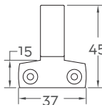
Front Profile
