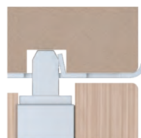
Tritus™ Flush Casement - Pair of sashes lock detail (TOP)
