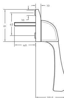
Side Profile
