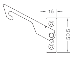
Right hand Restrictor shown
