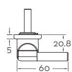
Top Profile
