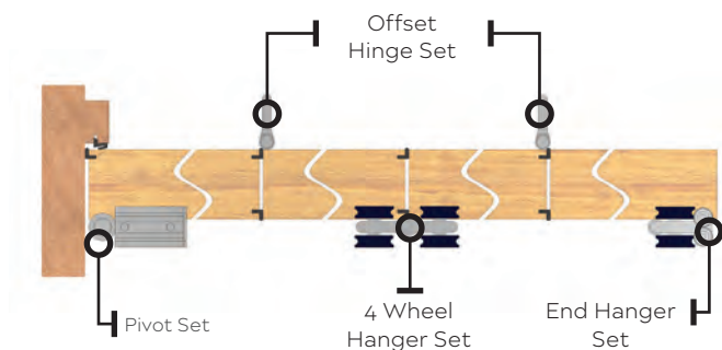
Securefold Pro Plan View
