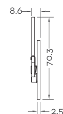
Side Profile
