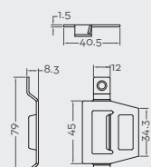
Side Profile Front Profile
