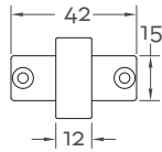
Front Profile
