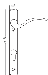
Front Profile
