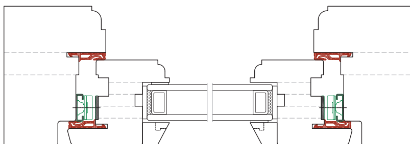
HIGH PERFORMANCE FLUSH WINDOW SYSTEM HORIZONTAL SECTION
