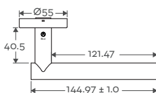
Top Profile
