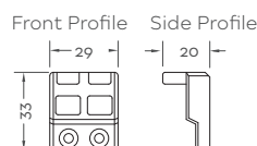
EBMK10 Used on single sash and connects to EBSK Keep as shown.
