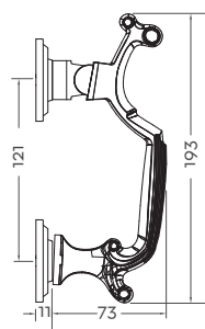
Front Profile
