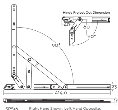
SPS16 Right Hand Shown, Left Hand Opposite.
