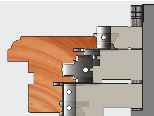
Double Sash Tilt & Turn Top view section
