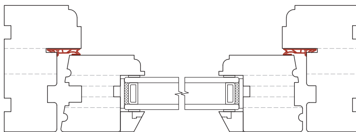
TRITUS WINDOW SYSTEM Horizontal Section
